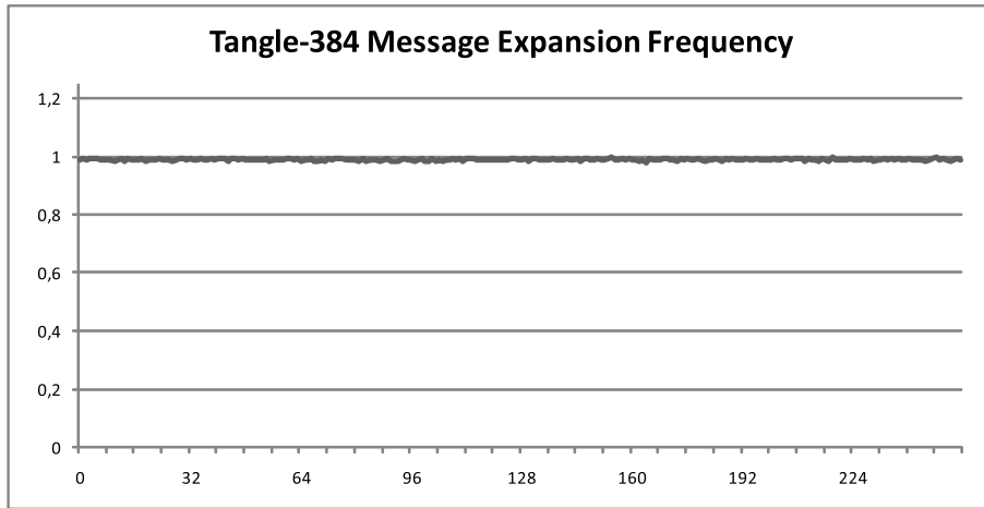
Figure 10: Message expansion byte frequency for Tangle-384
