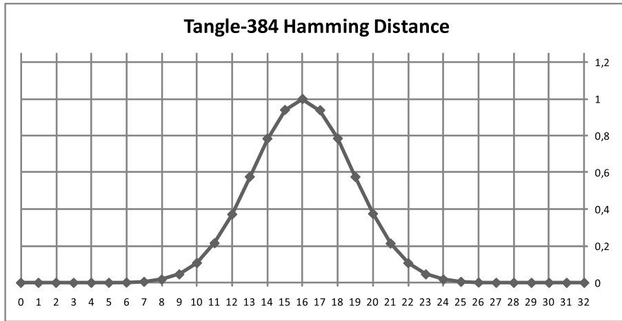
Figure 22: Block hash Hamming distance frequency for Tangle-384
