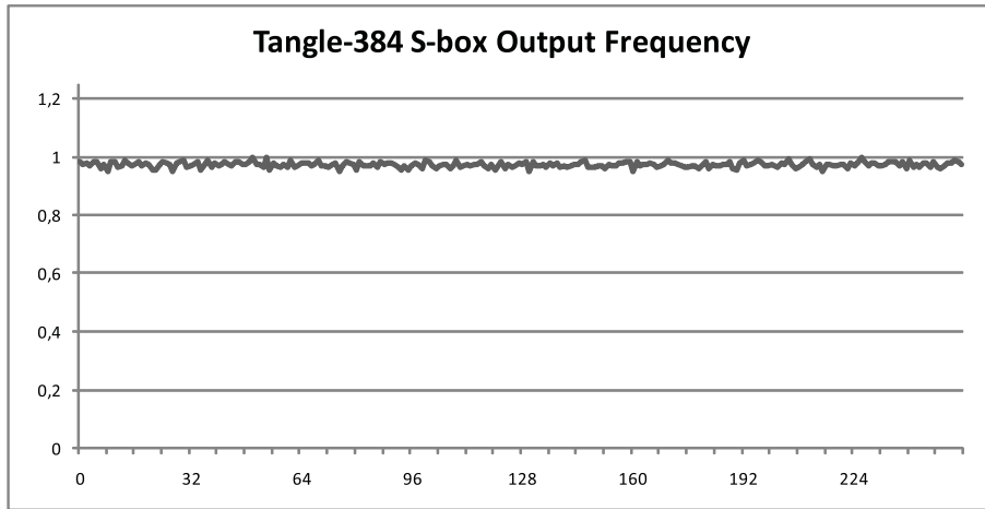
Figure 4: S-box output frequency for Tangle-384
