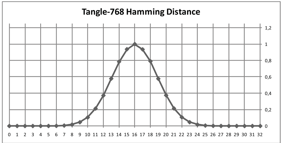
Figure 24: Block hash Hamming distance frequency for Tangle-768
