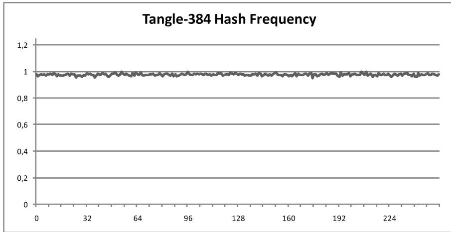
Figure 16: Block hash byte frequency for Tangle-384
