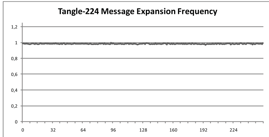
Figure 8: Message expansion byte frequency for Tangle-224
