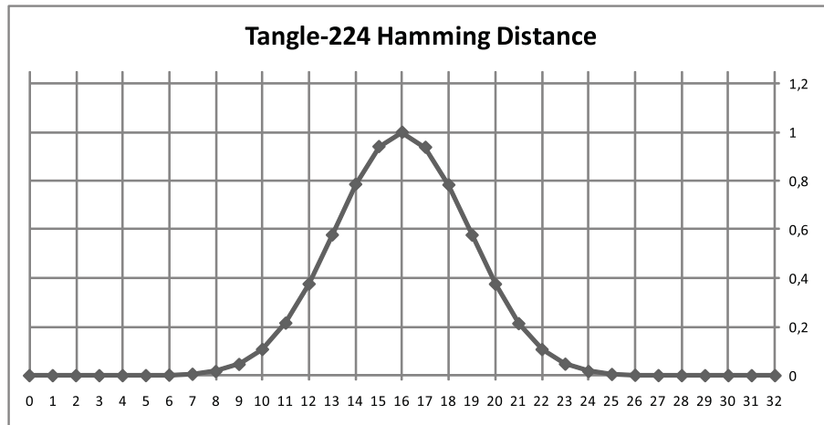
Figure 20: Block hash Hamming distance frequency for Tangle-224
