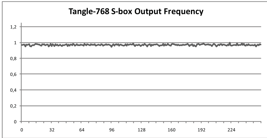
Figure 6: S-box output frequency for Tangle-768
