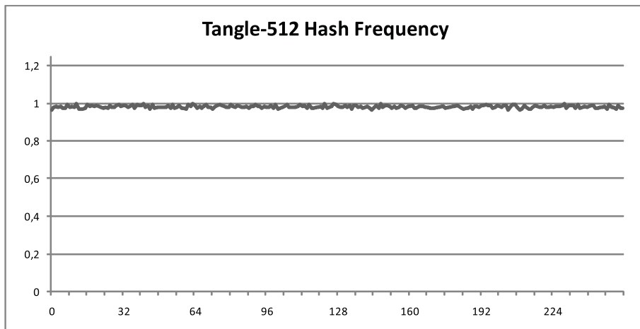
Figure 17: Block hash byte frequency for Tangle-512
