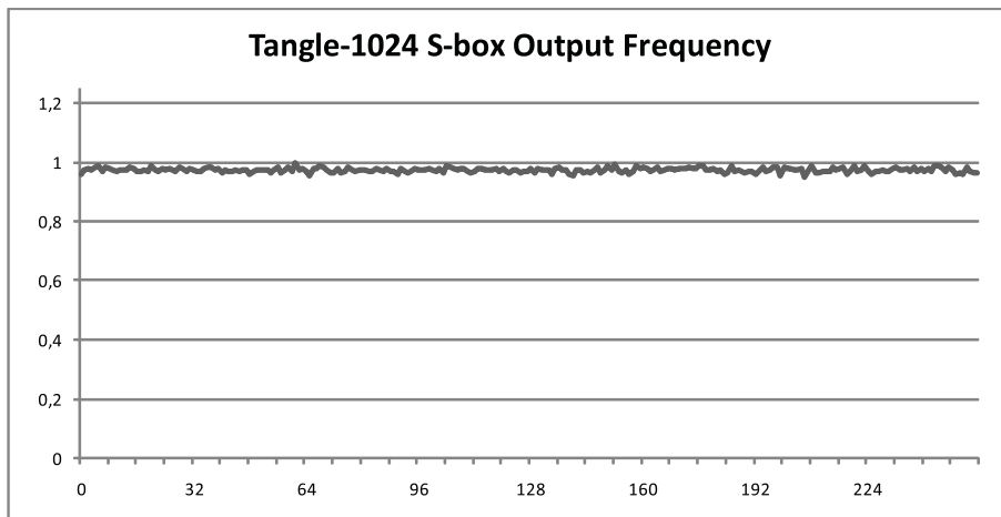
Figure 7: S-box output frequency for Tangle-1024
