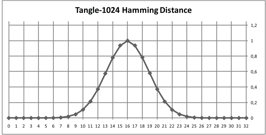
Figure 25: Block hash Hamming distance frequency for Tangle-1024
