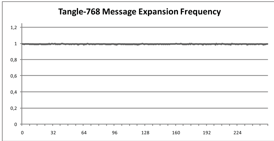
Figure 12: Message expansion byte frequency for Tangle-768
