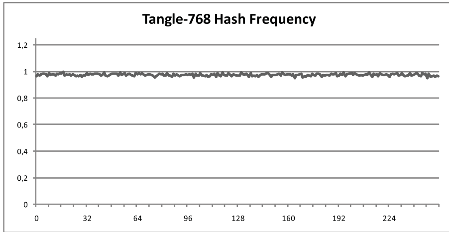
Figure 18: Block hash byte frequency for Tangle-768
