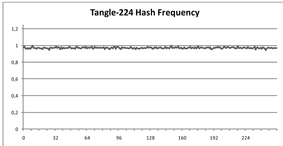
Figure 14: Block hash byte frequency for Tangle-224
