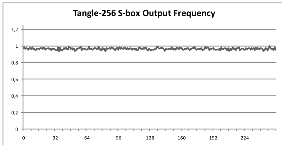
Figure 3: S-box output frequency for Tangle-256
