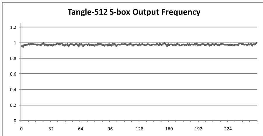
Figure 5: S-box output frequency for Tangle-512
