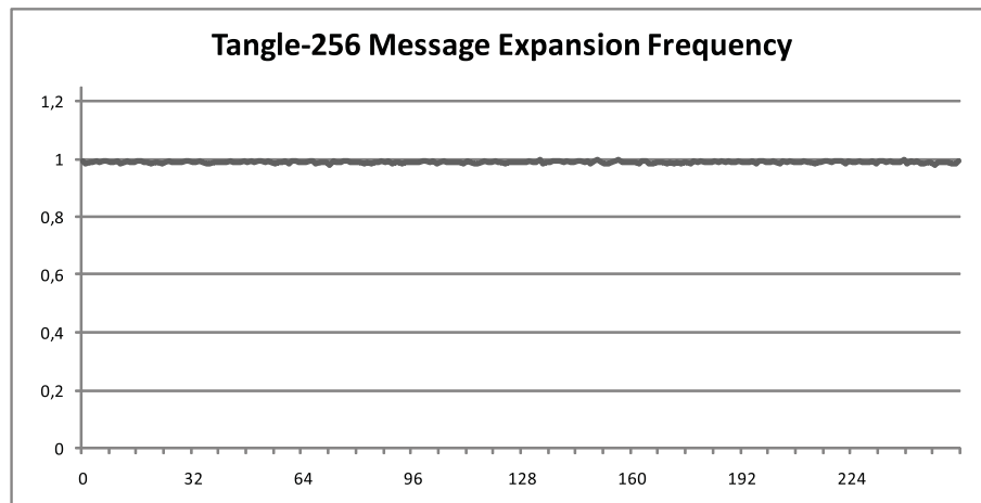
Figure 9: Message expansion byte frequency for Tangle-256
