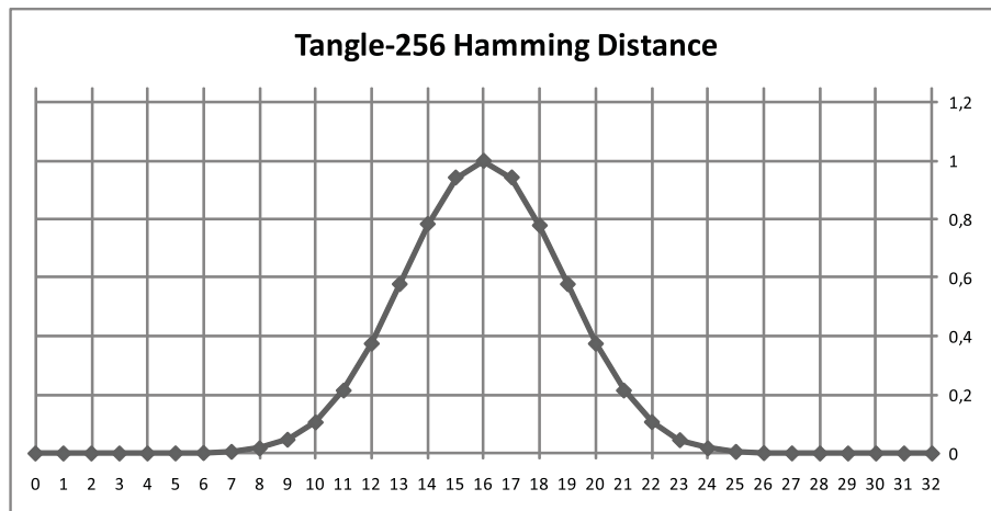
Figure 21: Block hash Hamming distance frequency for Tangle-256
