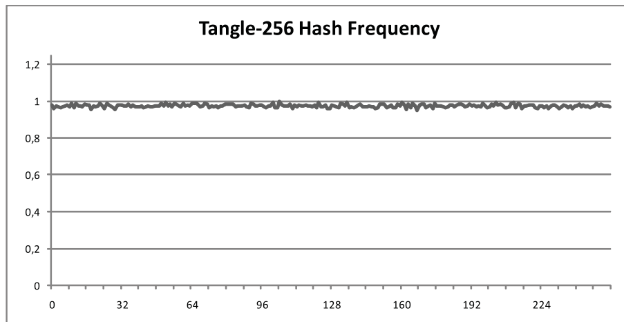
Figure 15: Block hash byte frequency for Tangle-256
