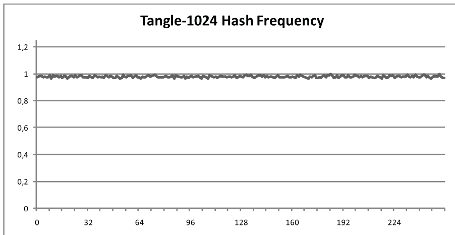
Figure 19: Block hash byte frequency for Tangle-1024
