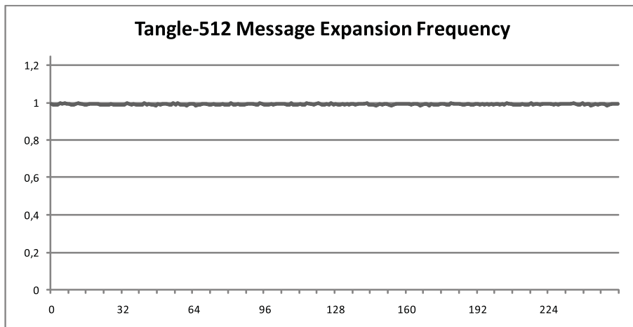
Figure 11: Message expansion byte frequency for Tangle-512
