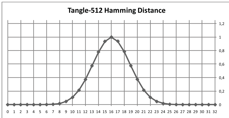
Figure 23: Block hash Hamming distance frequency for Tangle-512
