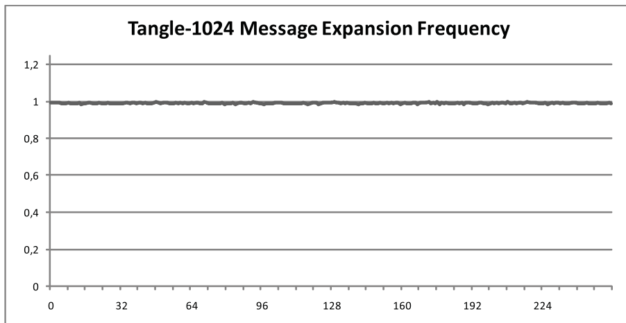
Figure 13: Message expansion byte frequency for Tangle-1024
