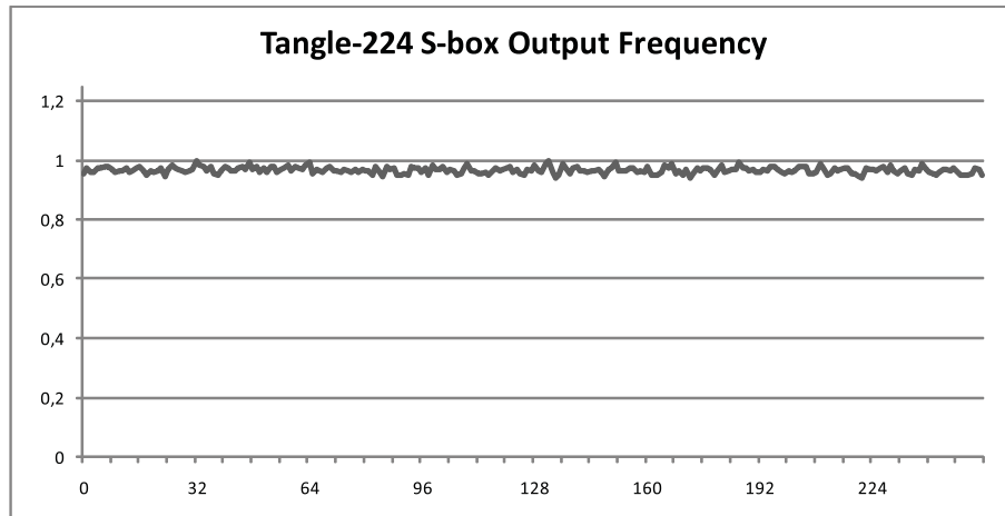
Figure 2: S-box output frequency for Tangle-224
